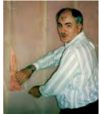
Photograph 2 Interior basement stud framing insulated with fiberglass batts and covered with a polyethylene vapor barrier
