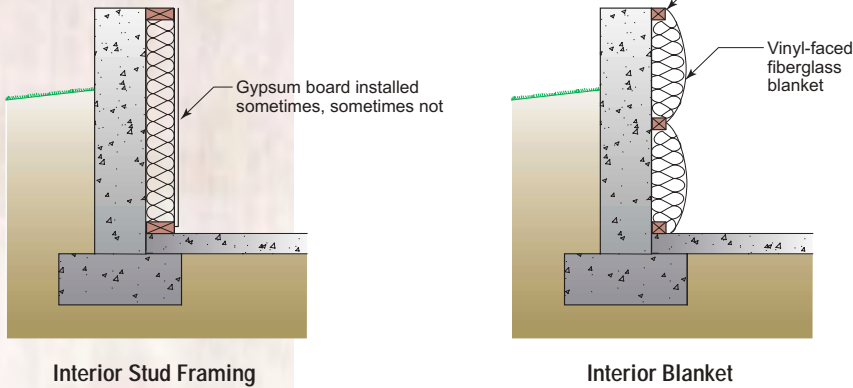
Figure 3 Interior insulation approaches
