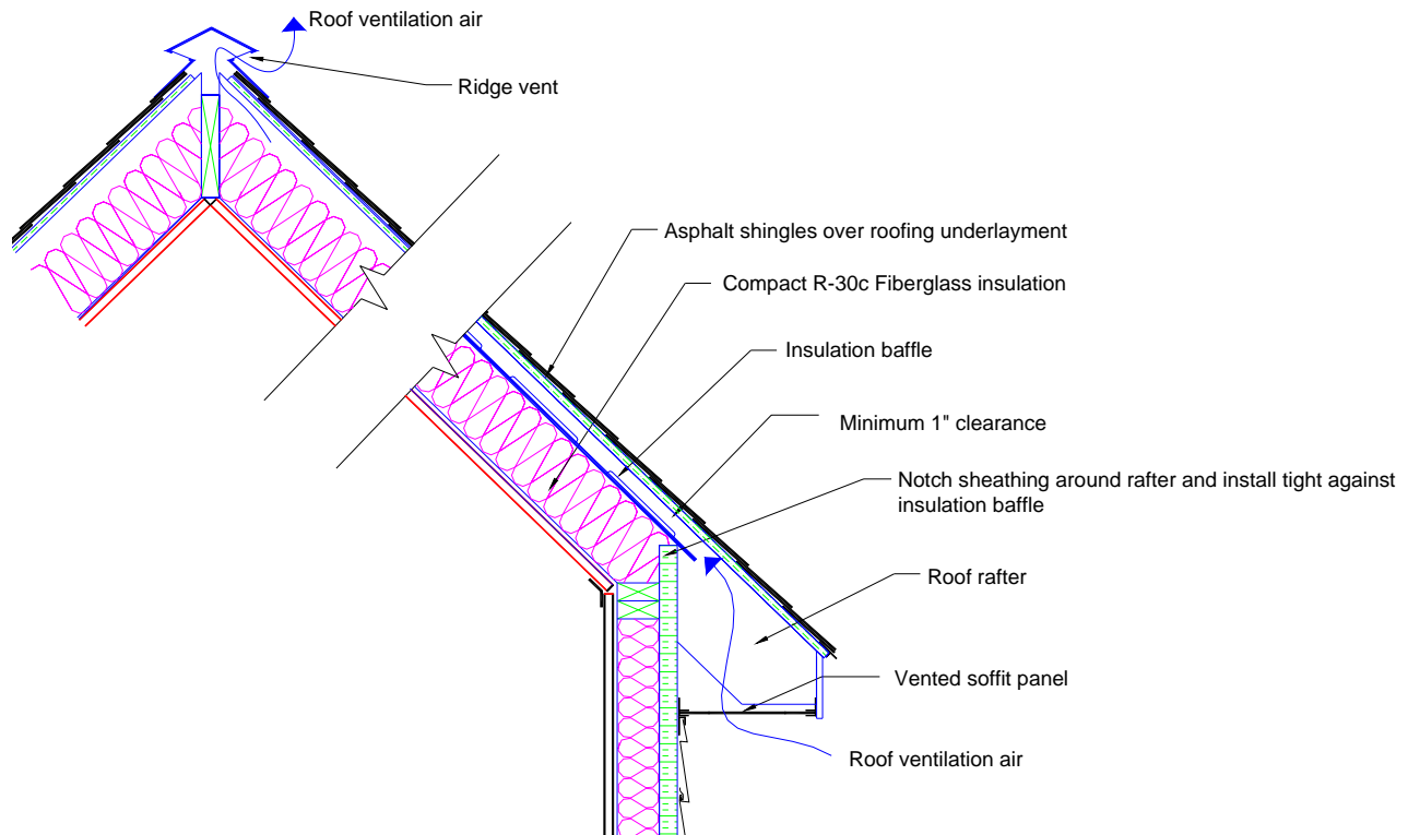
Figure 6. Correct method for insulating a vaulted ceiling.
