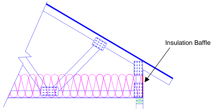
Figure 3. A high heel roof truss allows for a uniform height of insulation to be placed over the entire ceiling, thereby avoiding a potential cold spot at the perimeter of the wall.
