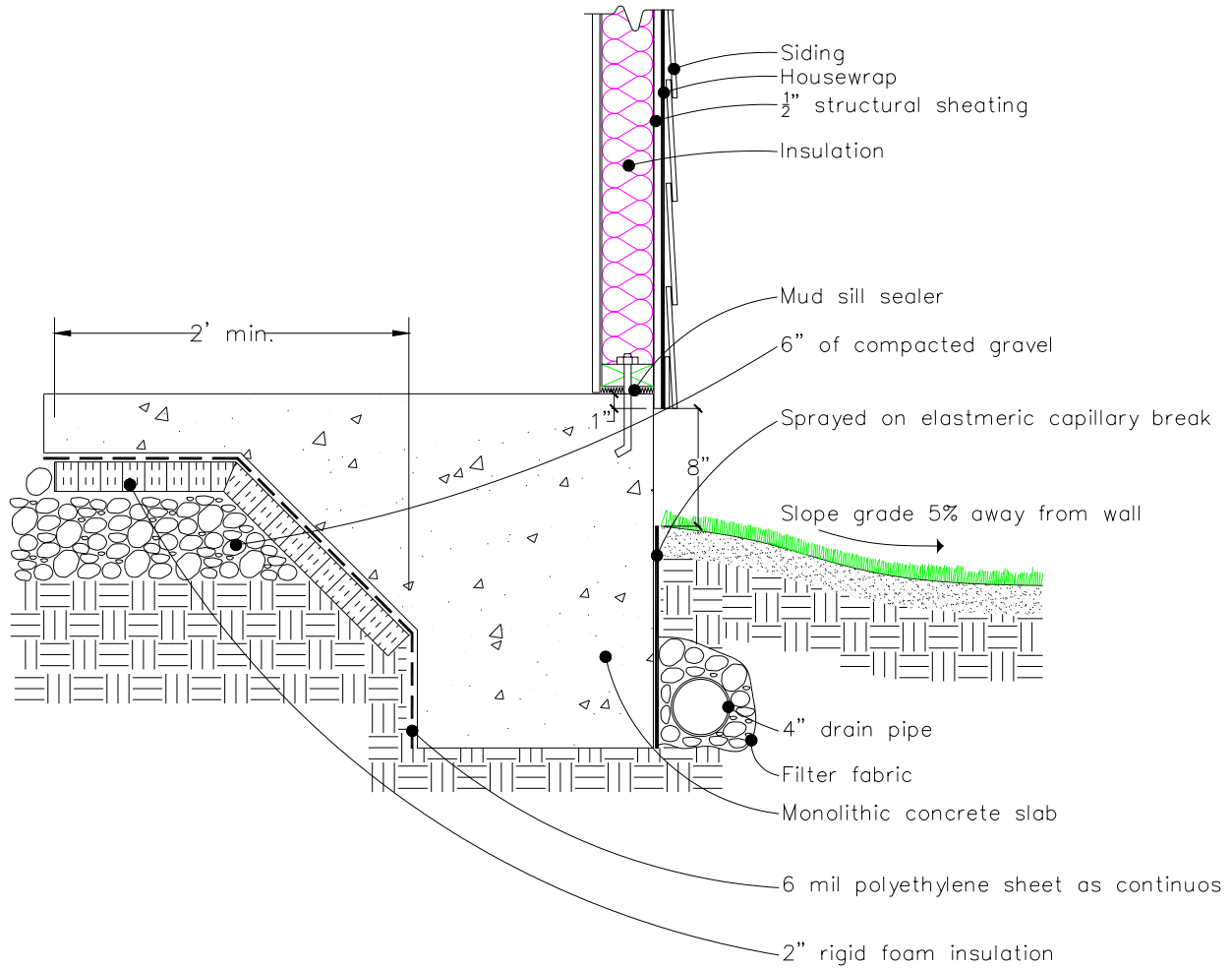
Figure 5. Insulating below a slab-on-grade foundation at the perimeter prevents heat loss in the slab area where it is greatest.
