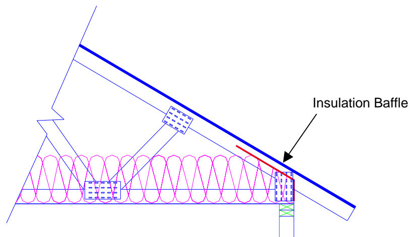
Figure 2. A baffle attached to the top plate at the roof perimeter prevents insulation from entering into the soffit. It should be used between every roof truss if blown insulation is used in the attic.
